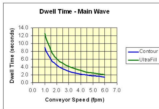
Dwell time comparison between coN2tour and UltraFill nozzles
